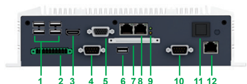
Front view of Magelis HMIBSU Universal
