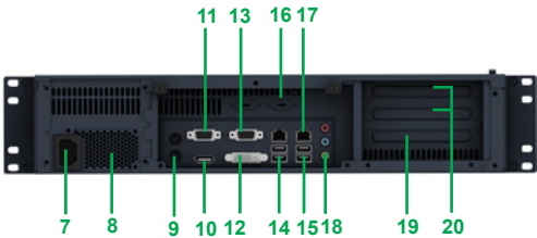
Rear view of Universal Magelis Rack PC
