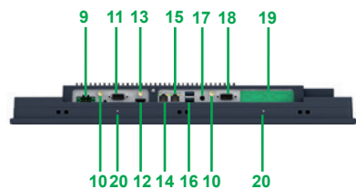
19" underside view
