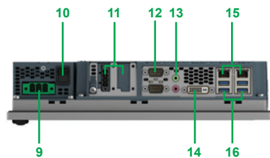
Underside view
