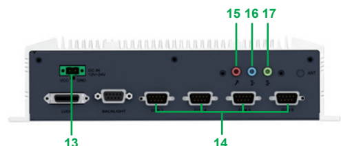
Rear view of Magelis HMIBSU Universal
