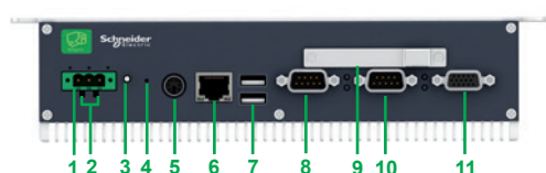
Front view of Magelis HMIBSO Optimized
