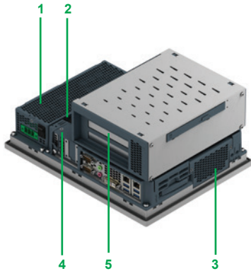
Rear view
