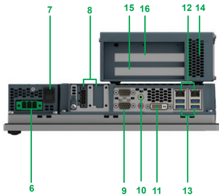
Underside view
