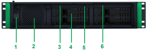
Front view of Universal Magelis Rack PC
