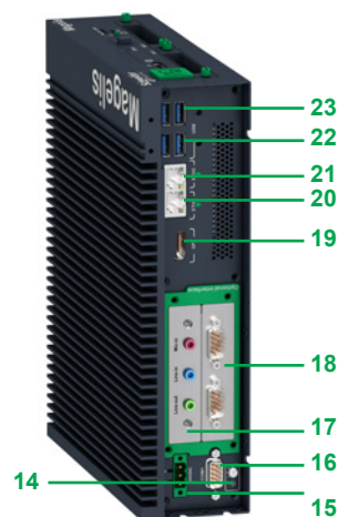
Underside view of Magelis Modular Box PC, 2 expansion slots
