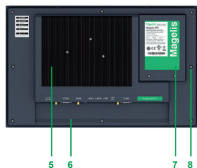
19" rear view
